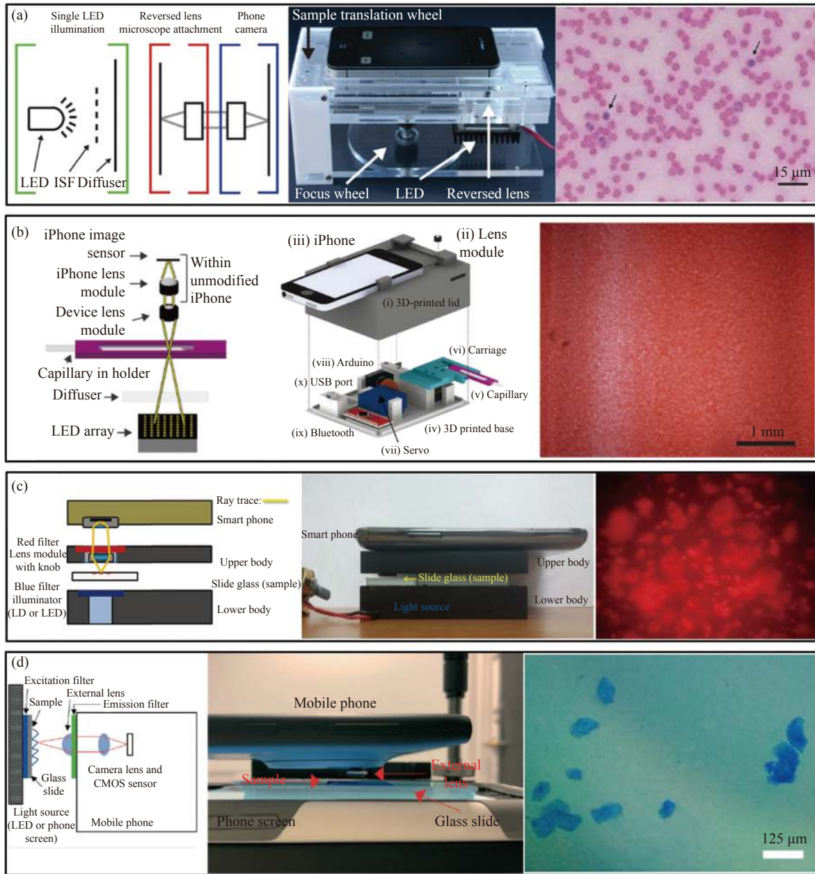
Fig.8 Schematic diagram of various self-correcting intelligent mobile phone platform microscopic imaging systems based on inverted mobile phone lenses. (a) Schematic diagram of the smartphone platform-based microscope proposed by Switz et al [76] ; (b) Schematic diagram of the smartphone platform-based microscope proposed by D'Ambrosio et al [77] ; (c) Schematic diagram of the smartphone platform-based microscope proposed by Kim et al [78] ; (d) Schematic diagram of the microscope based on smartphone platform by Kheireddine et al [79]
