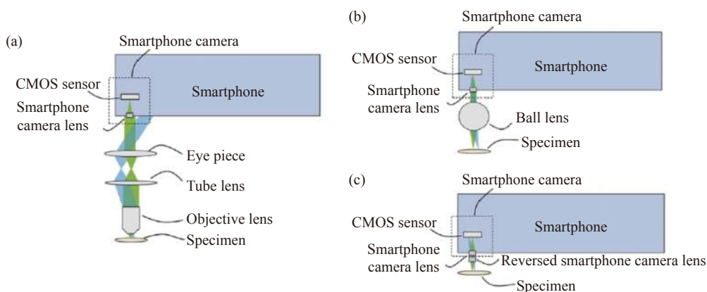
图 2 基于智能手机平台的显微系统中的各种物镜类型。(a) 标准显微成像光路; (b) 定制化单透镜; (c) 倒置手机摄像头镜头的自校正显微光路 Fig.2 Various objective lens types in microscope system based on smartphone platform. (a) Standard microscope objective and eyepiece; (b) Customized lens; (c) Self-correcting microscopic optical path of inverted camera lens of smart phone
